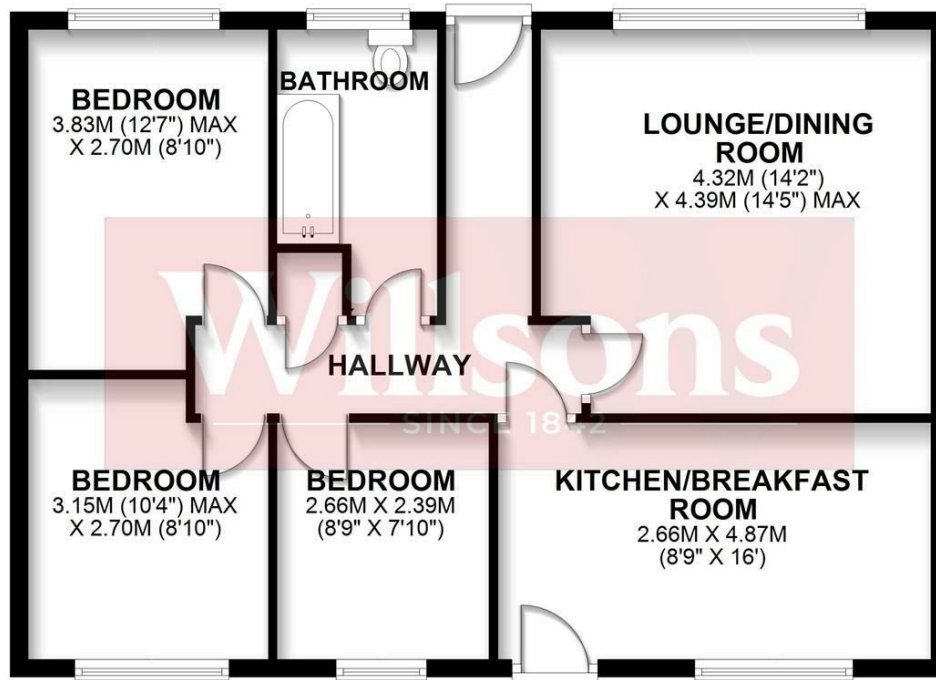
FLOOR PLAN
